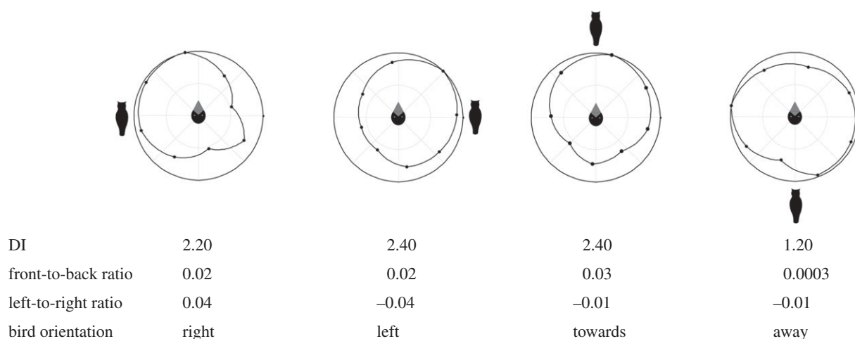
Figure 3. Sample polar plots of acoustic radiation of yellow-rumped warbler antipredator calls. Points on each plot represent the amplitude as measured at each of the eight microphones, connected by linear interpolation. All polar plots are in decibels, with the loudest value normalized to 0 dB (outermost circle on the plot) and an origin at -12 dB. All plots are oriented so that the bird's head is facing upward; the relative position of the owl is indicated by an owl icon.
